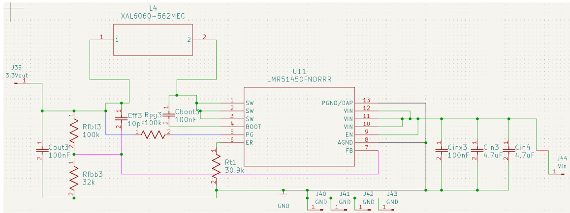
Figure 26: LMR51450 Buck Converter
