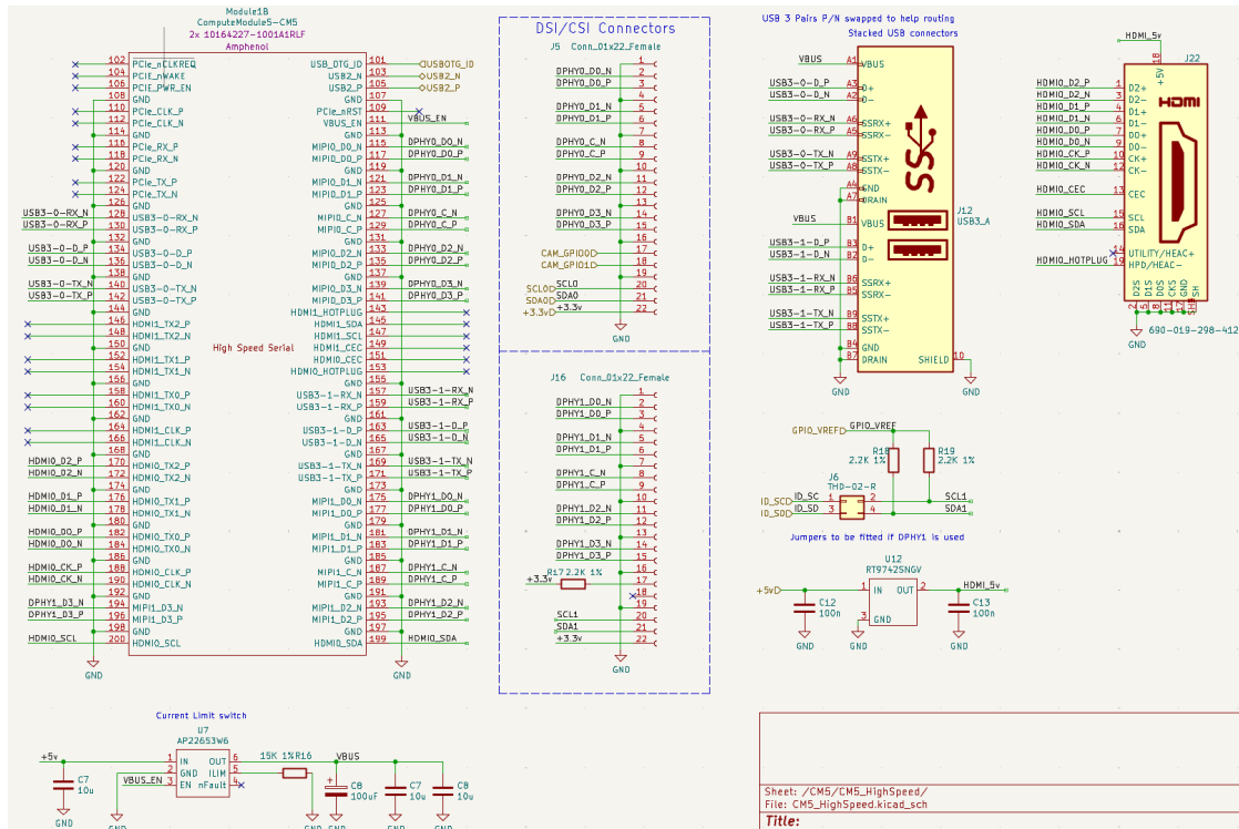
Figure 20: High-level Carrier Board Design
