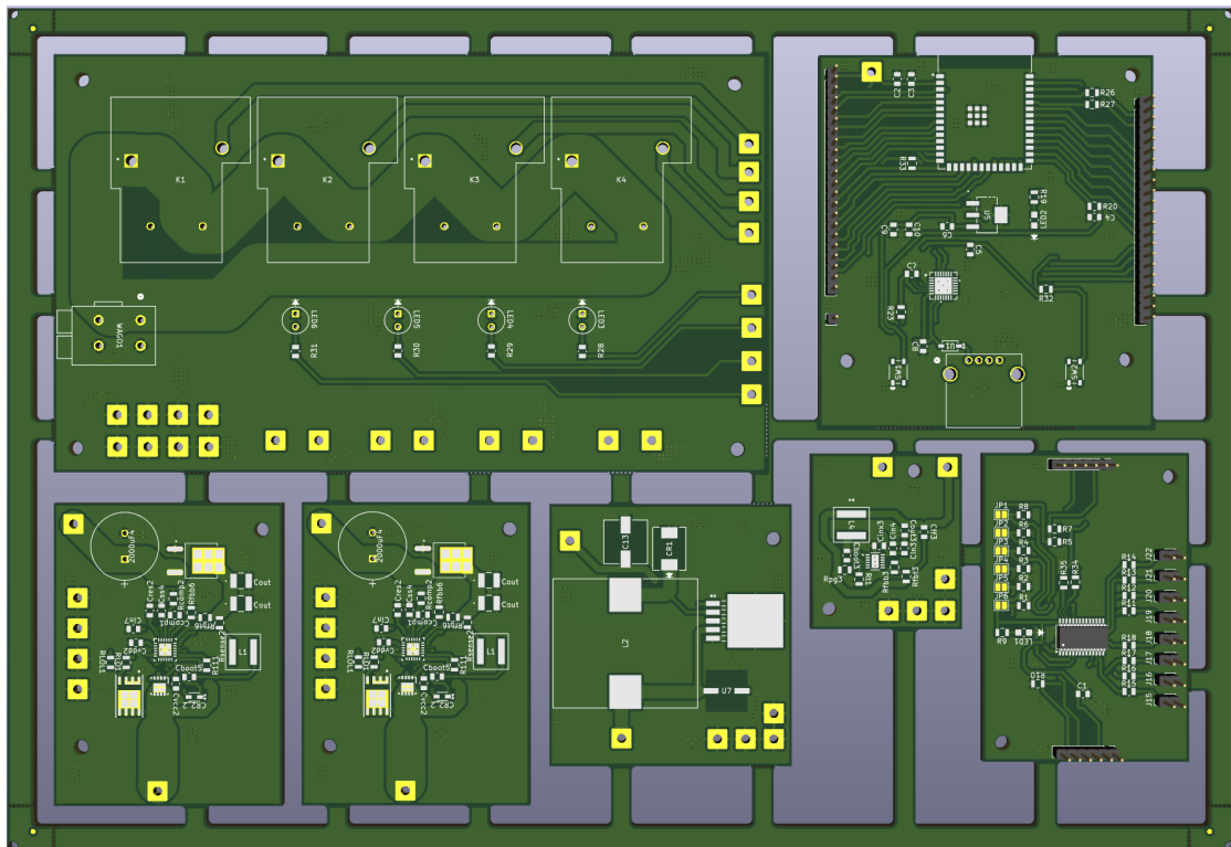
Figure 52: Custom Pannelized PCB Render
