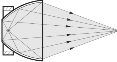
Figure 9. Ellipsoidal reflector diagram showing how light from the first focal point reflects to the second focal point. Adapted from [18].
