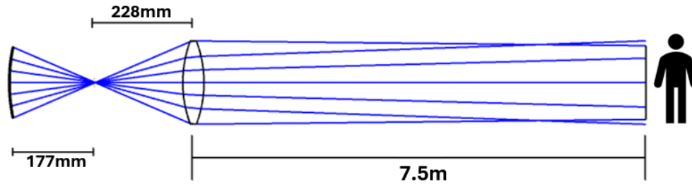
Figure 4: (from left to right) Illumination reflector, gate, and lens; pointing towards subject
