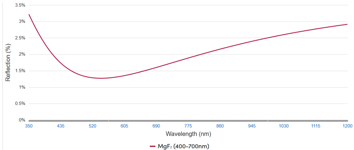
Figure 14: Reflectance (%) of an MgF2 Coated Lens
