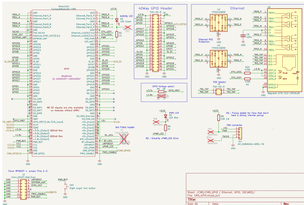
Figure 22: GPIO Carrier Board Schematic
