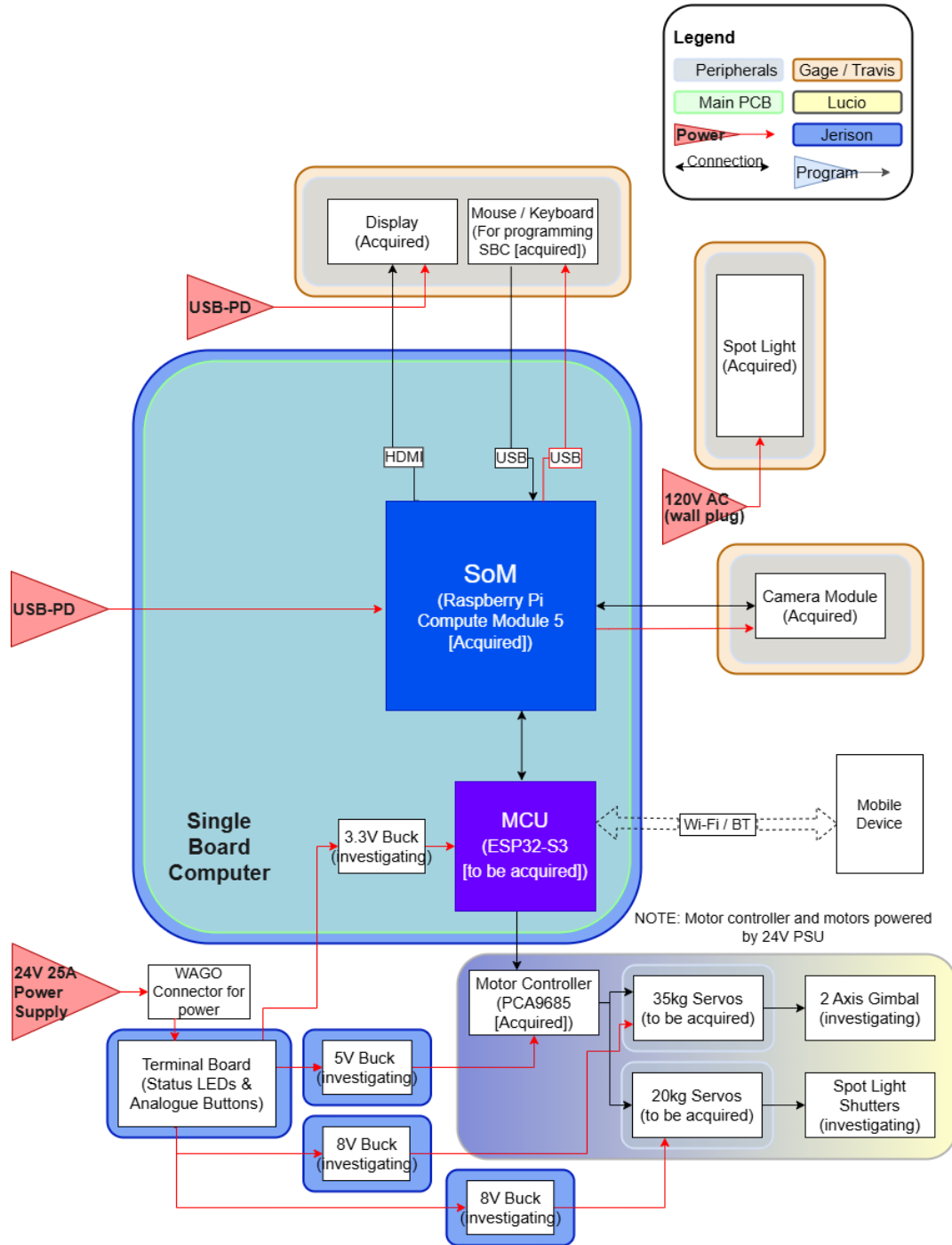
Figure 6.0: Hardware Block Diagram
