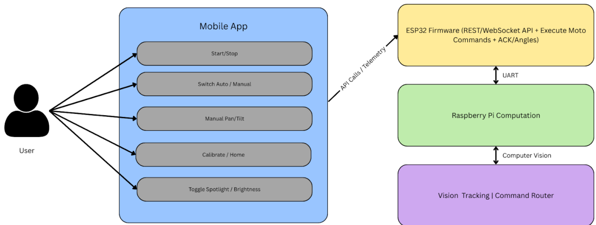
Figure 37: User Interaction Use Case Diagram
