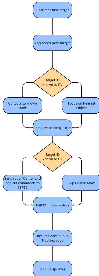
Figure 42: Continuous Tracking Loop Flowchart
