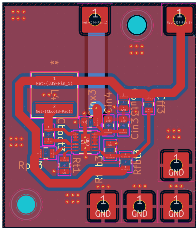
Figure 48: 7.4V Buck PCB
