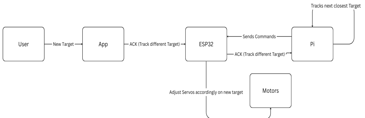
Figure 41: Target Selection Sequence
