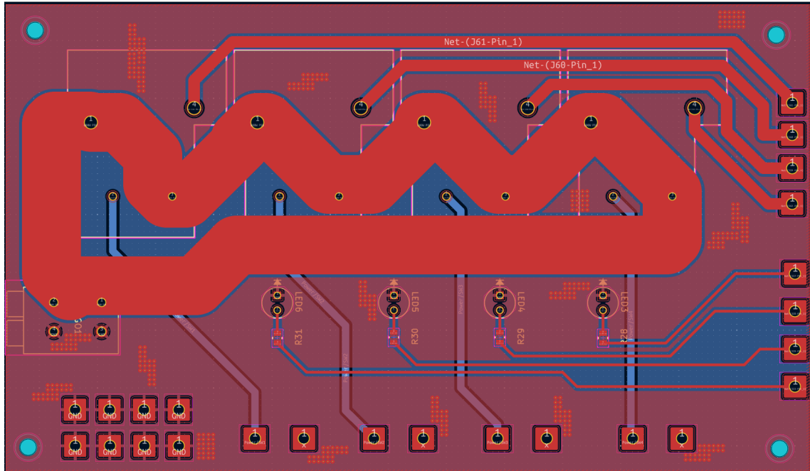
Figure 51: Custom Terminal Board PCB
