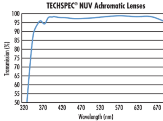
Figure 15: Transmission of a UV-VIS Coated Lens
