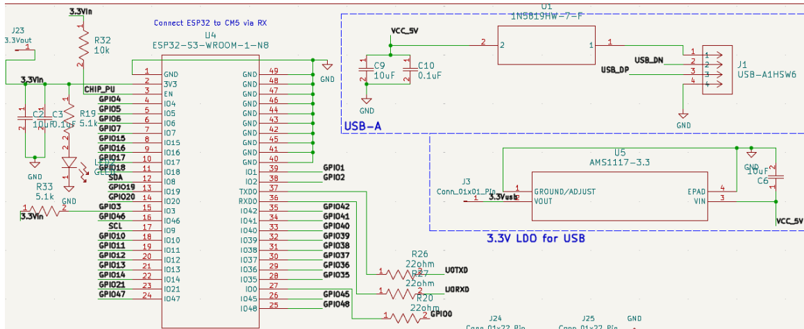
Figure 23.1: ESP32 Schematic
