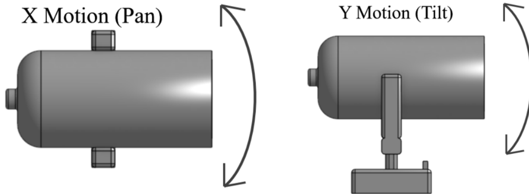
Figure 3: Gimbal motion axes of the S.T.A.R. system. The left view shows rotation about the X-axis (pan), and the right view shows rotation about the Y-axis (tilt).
