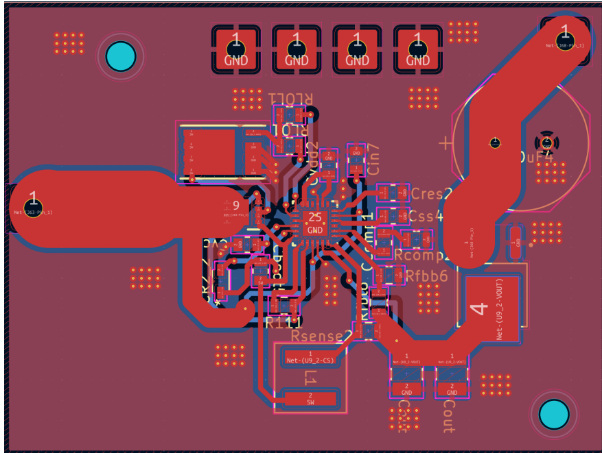
Figure 48: 7.4V Buck PCB
