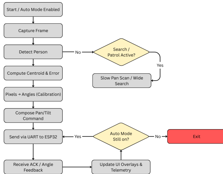
Figure 32: Continuous Tracking Loop Flowchart
