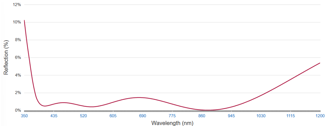
Figure 16: Reflectance (%) of a VIS-NIR Coated Lens
