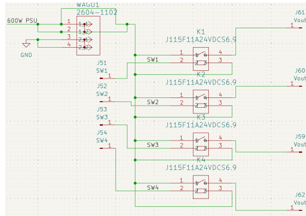
Figure 30: Terminal Board Schematic
