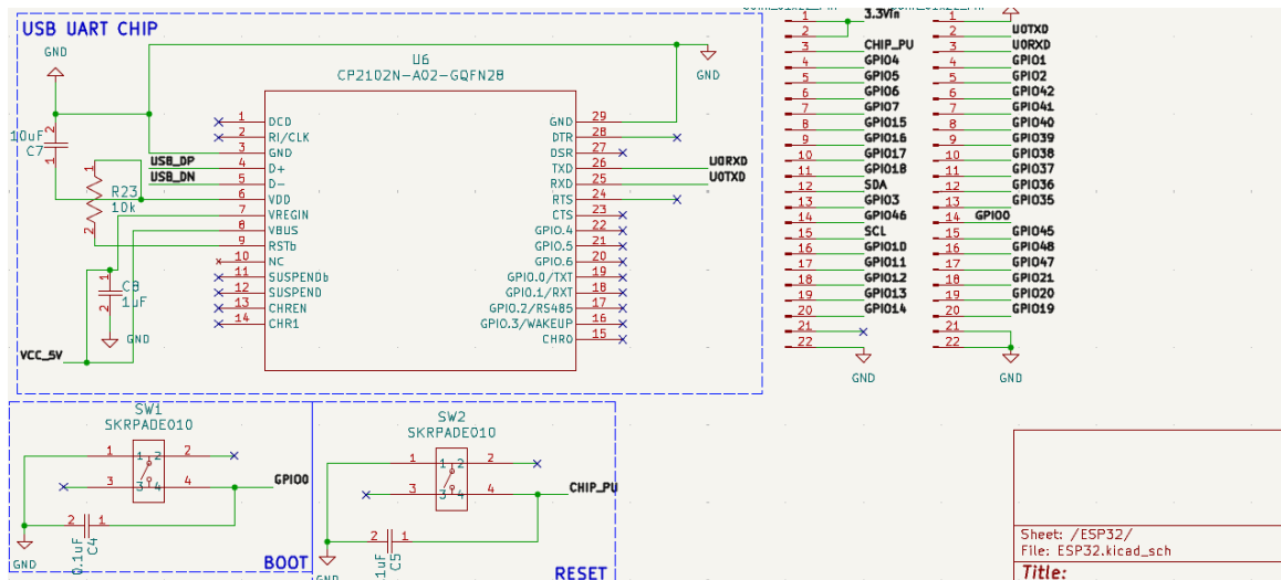
Figure 23.2: ESP32 Schematic
