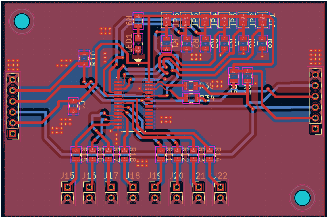
Figure 50: Custom PCA9685 PCB
