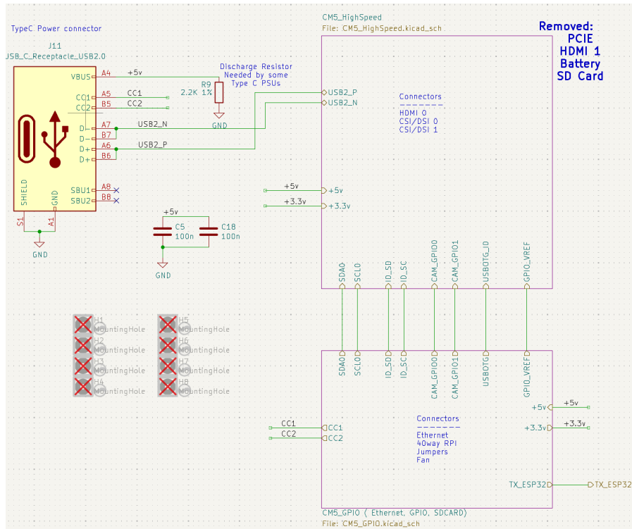
Figure 20: High-level Carrier Board Design
