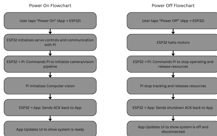
Figure 40: System Power-On and Power-Off Flowcharts
