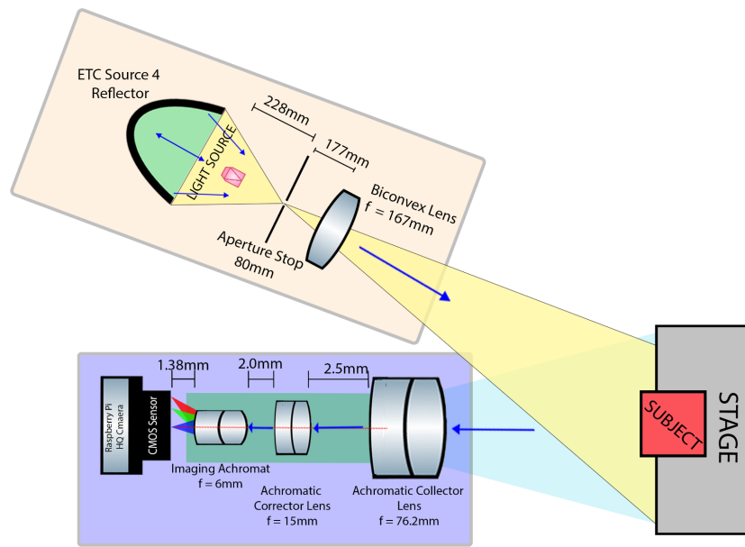
Figure 1: Optical Schematic
