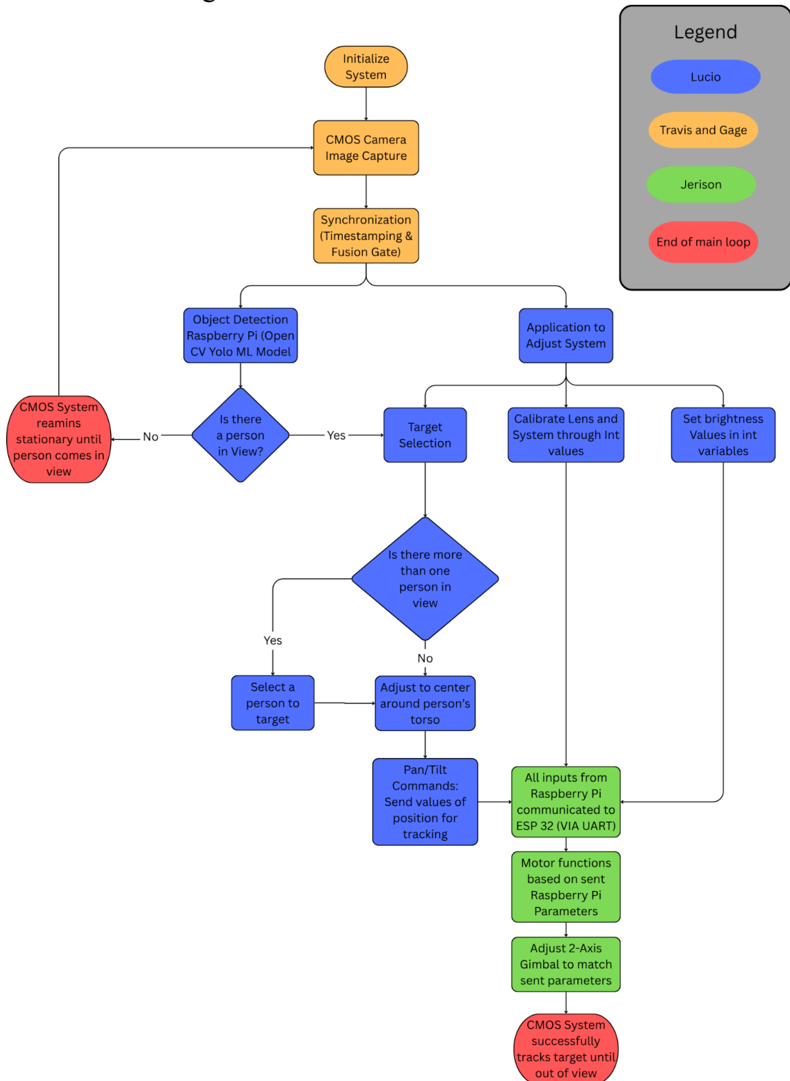
Figure 6.1: Software Block Diagram
