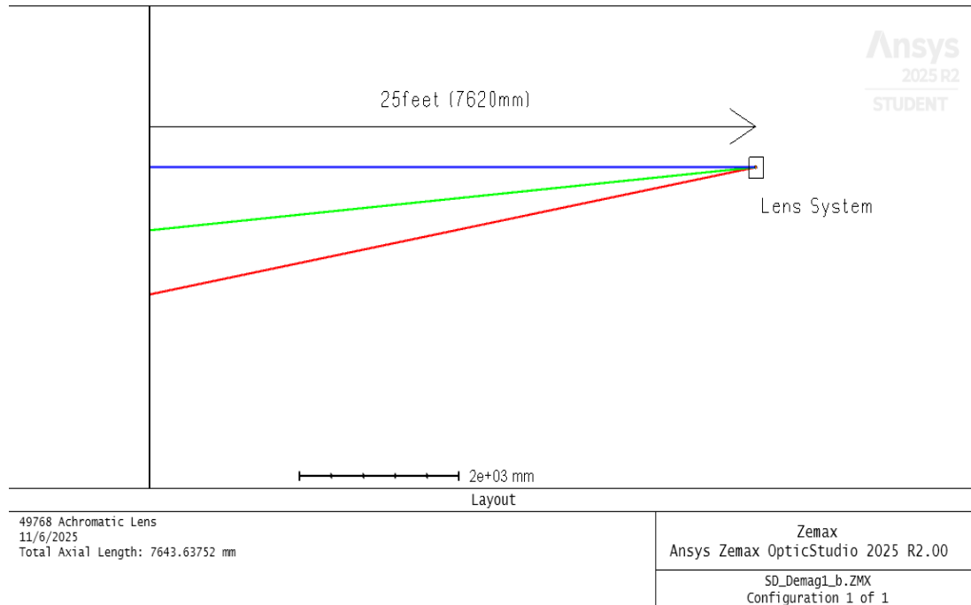
Figure 17.1 Zemax Simulation of Selected COTS Lenses.
